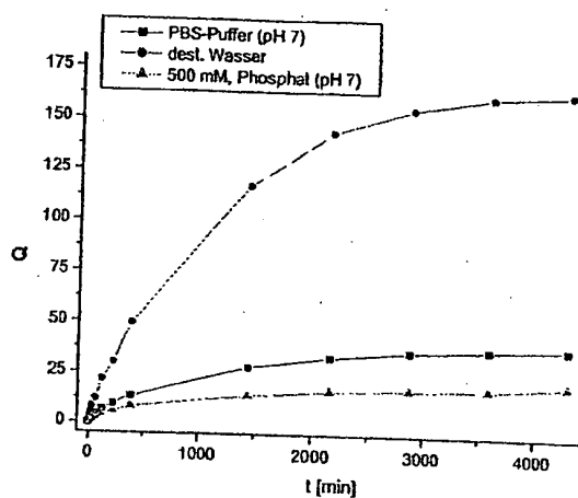
Fig. 13: Comparison of the swelling characteristics of a ball-milled synthesised hydrogel based on acrylamide/acrylic acid and MDA (molar ratio = 204/141/1) in distilled water, in PBS and 500 mM phosphate buffer
